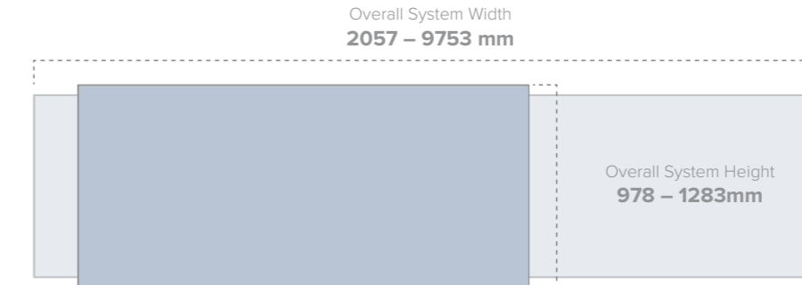
Horizontal Orientation Overall System Width 2057 – 9753 mm
